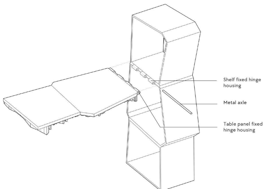
Figure 23: Hinge mechanism
